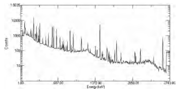
Figure 1. A typical gamma-ray spectrum of the soil sample
